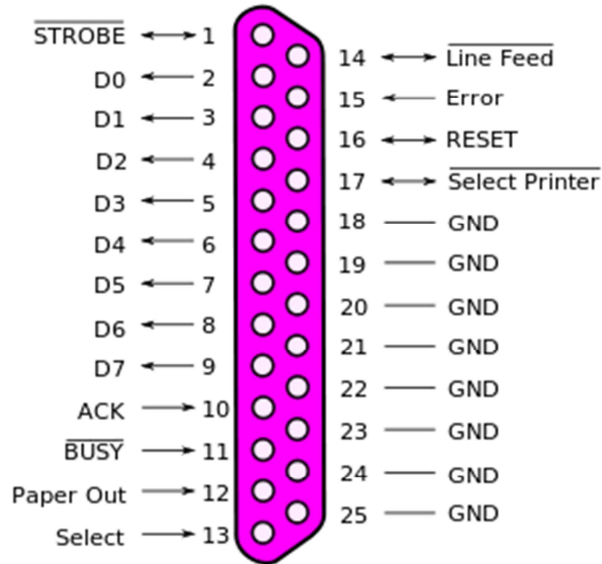
Figure 1 http://en.wikipedia.org/wiki/File:Parallel_port_pinouts.svg
